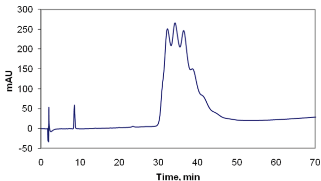
Figure 2. Chromatogram of 1 showing free paclitaxel (~9 min) and a series of peaks (attributed to differing degrees of PEGylation) corresponding to dendrimer 1 .
