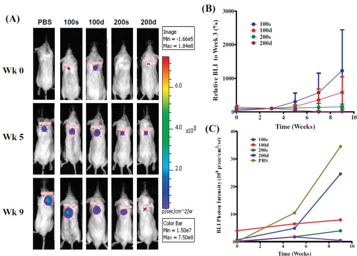
Figure 6. BLI evaluation of the therapeutic efficacy of 1 in SCID mice bearing PC-3-h-luc xenografts. (A) Representative BLI images of four treatment groups and PBS control. The photon intensity of the BLI images is shown on the same scale. (B) Comparative presentation of BLI signals of the four treatment groups. The relative BLI signals at the given week were normalized to the data at week 3 (set at 100%) for all individual mice. (C) Absolute BLI photon intensity quantification of the five tumor-bearing mice shown in (A).
